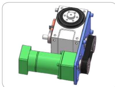
凸轮分割器带电机方案2 Cam Indexer with Motor Solution 2
